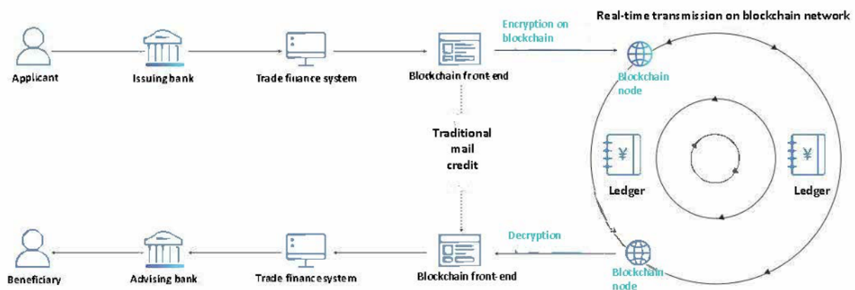
Exhibit 2.8 General framework of the blockchain solution for trade finance
