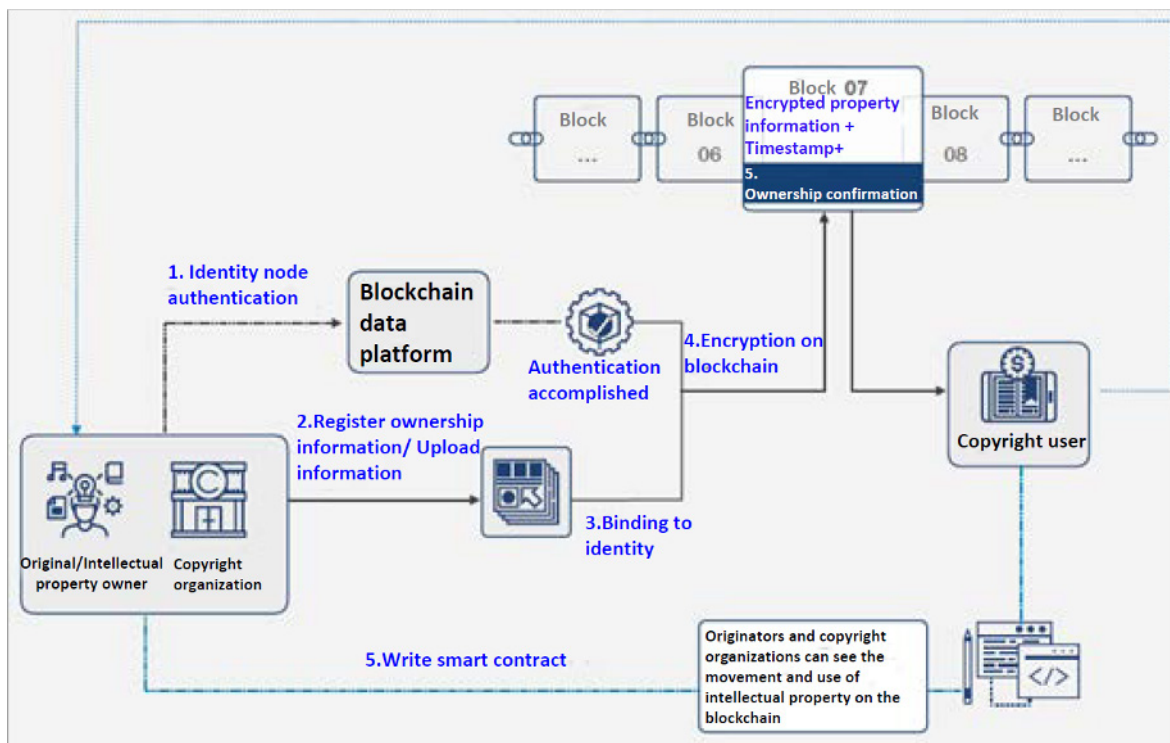
Exhibit 2.11 Blockchain-based solution for copyright protection
