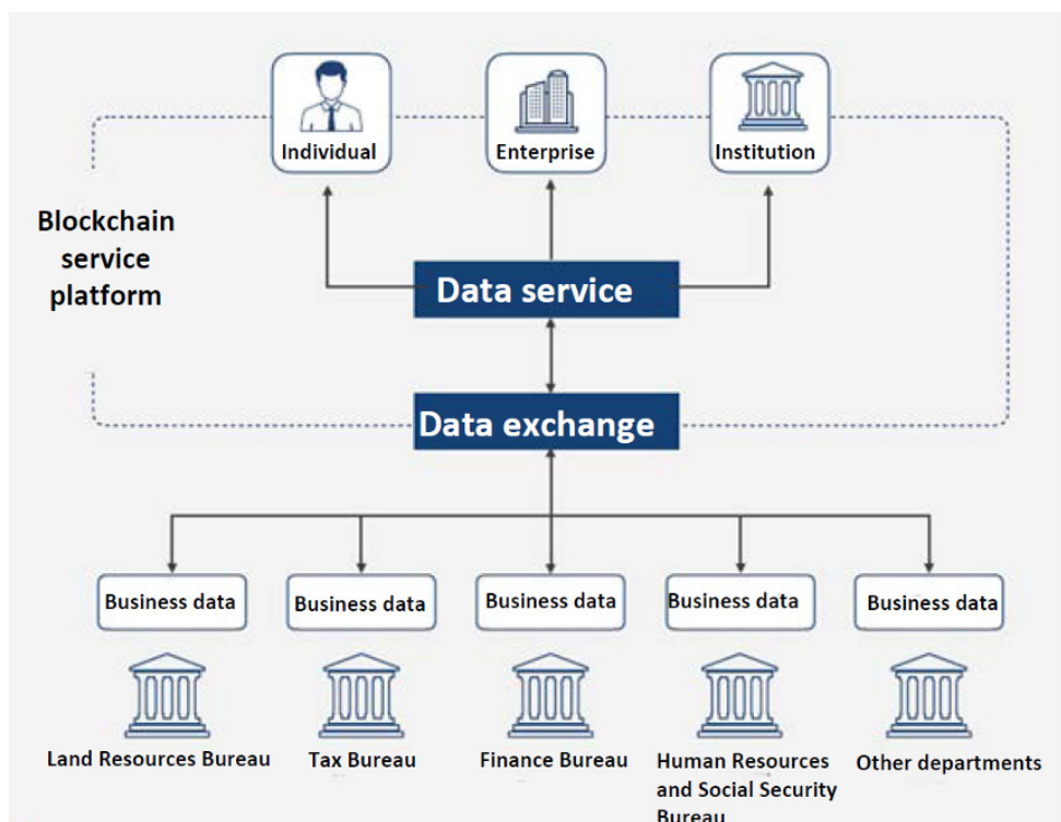
Exhibit 2.12 Blockchain-based information sharing for public service/government departments
